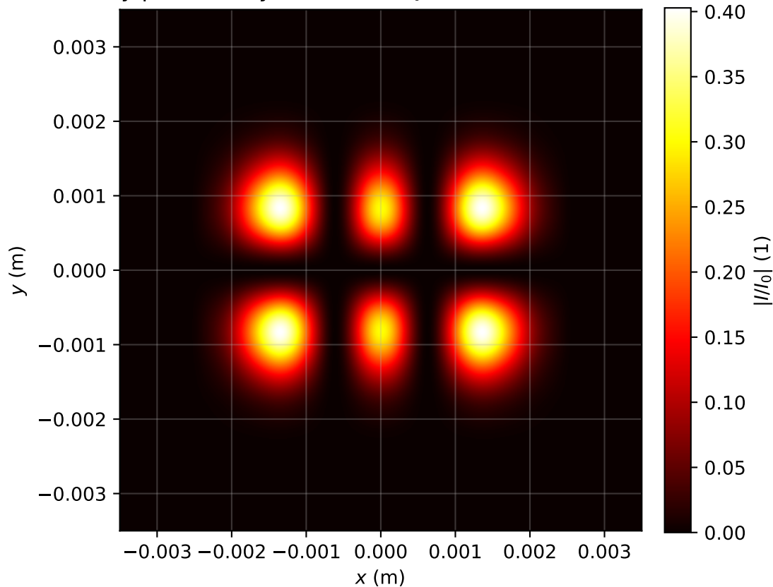
Intensity profile I(x, y, z = 2.786)/I_0 , P_{in}=1.0P_{cr} , artificial time
